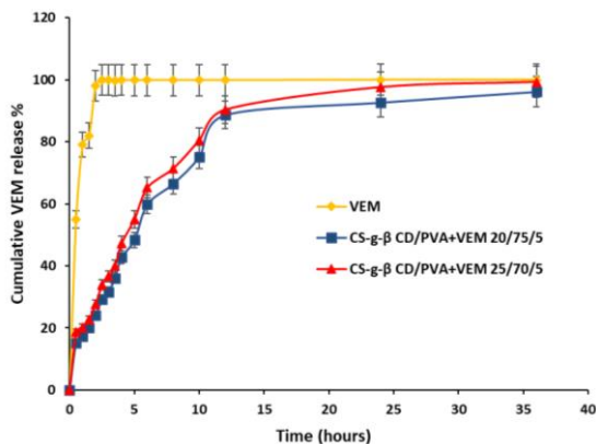
Fig. 8. Drug release of VEM. Data are mean \pm SD within \pm 2 (n = 3)
