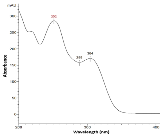
Fig. 4. Absorption spectra of VEM
