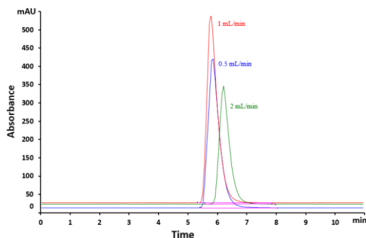
Fig. 3. Overlaid chromatograms of VEM samples with 12 mg/L concentration at different flow rates
