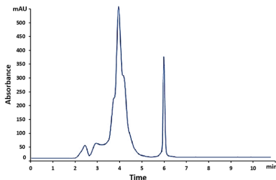
Fig. 5. Sample chromatogram for stability study
