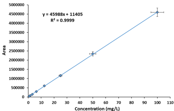
Fig. 6. Calibration graph for VEM over the range of 0.78-100 mg/L (area mean \pm SD, n = 3 ); SD: Standard Deviation
