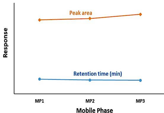
Fig. 1. The effect of mobile phase content to peak area and the retention time of VEM
