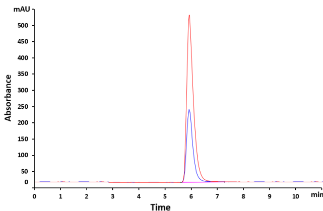
Fig. 2. Overlaid chromatograms of VEM samples with concentrations of 8 and 12 mg/L
